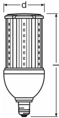
PARATHOM HQL LED 2000 lm 18 W/840 E27
