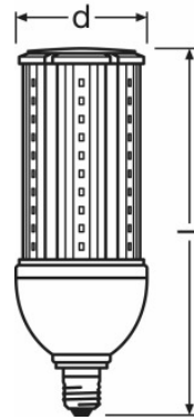
PARATHOM HQL LED 2500 lm 24 W/840 E27
