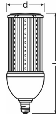
PARATHOM HQL LED 4000 lm 36 W/840 E27
